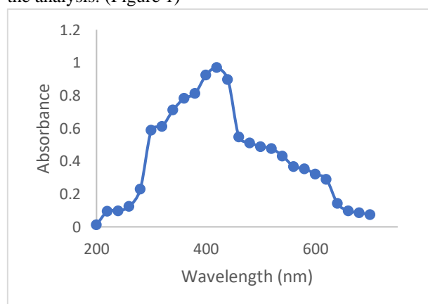
Figure 1: UV spectrum analysis of Methotrexate.
