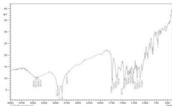
Figure 6: FTIR spectrum of Methotrexate and Tween
