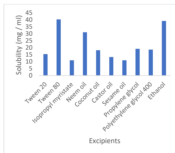
Figure 2: Graphical analysis of the solubility tests of Methotrexate.
