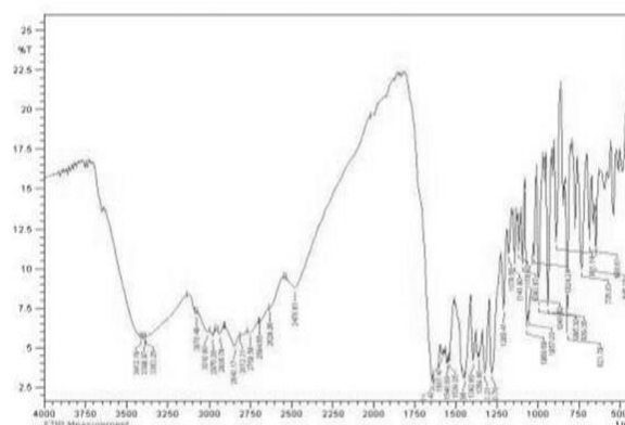
Figure 3: FTIR spectrum of pure drug Methotrexate.
