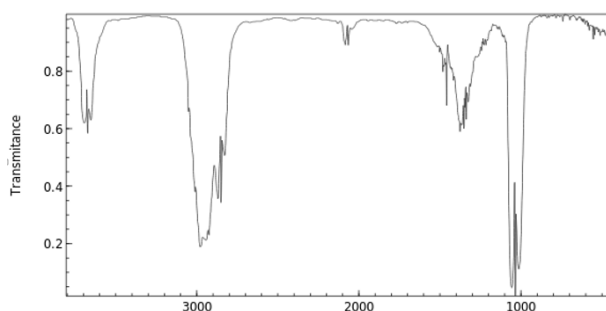
Figure 5: FTIR analysis of Tween 80
