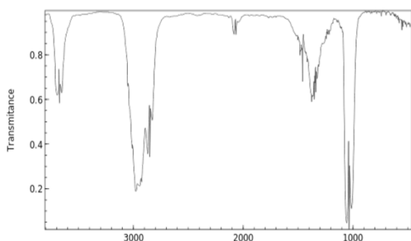
Figure 4: FTIR analysis of Methanol
