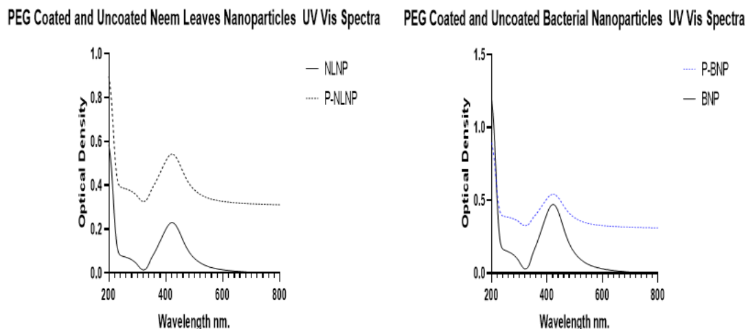
Fig.1. UV-Visible Spectroscopy analysis of PEG coated and uncoated NLNP and BNP Silver Nanoparticles: P-NLNP =PEG coated Neem Leaf Nanoparticles, P-BNP= PEG coated Bacterial Nanoparticles, NLNP = Neem Leaf Nanoparticles and BNP = Bacterial Nanoparticles.
