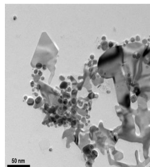
Fig. 2. (b) PEG coated BNPs
