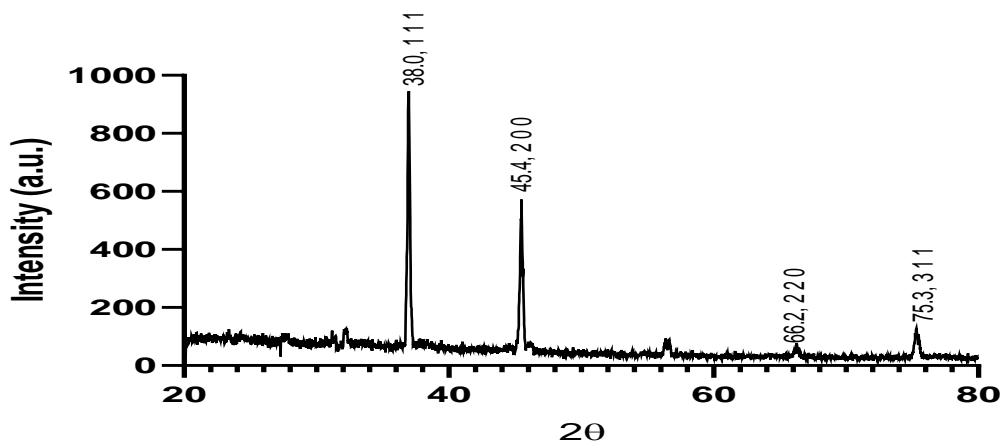
Fig. 3. (b) XRD Spectra of BNP
